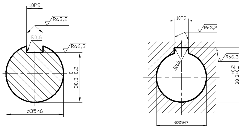
Keyway in shaft and in hub - example of dimensioning
